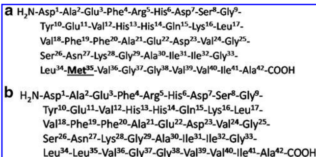
FIG. 1. Met at residue 35 of AB (1–42) is key to oxidative stress associated with this peptide. Amino-acid sequence of amyloid (1–42) peptide (a) showing Met at position 35. Met is key to amyloid (1–42)-induced oxidative stress and neurotoxicity. In the current study, the Met of A \beta (1–42) in APP was replaced by Leu (b). Residue 35 in both peptides is underlined. A \beta , amyloid-beta; APP, amyloid precursor protein; Lec/L, leucine; Met/M, methionine.
