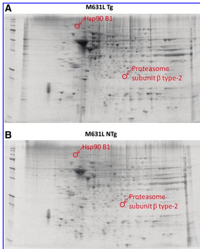
FIG. 2. Proteomics was used to identify proteins of differential levels in brain from M631L Tg vs. M631L NTg mice. Representative 2D-gel images of the proteins isolated from the brain of (A) M631L Tg and (B) M631 NTg mice. Differentially expressed protein spots in M631L Tg mice are labeled with protein identifications obtained from nanospray ESI-MS/MS analyses. 2D, two-dimensional; ESI, electrospray ionization; MS, mass spectrometry; NTg, non-transgenic; Tg, transgenic. (To see this illustration in color the reader is referred to the web version of this article at www.liebertpub.com/ars .)
